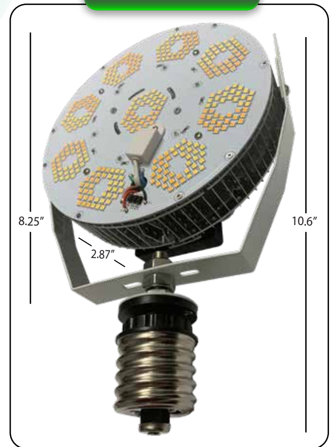
Dimensional Diagram
