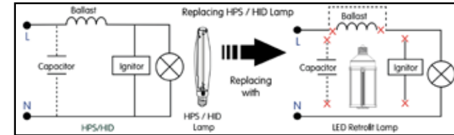
Wiring Diagram
